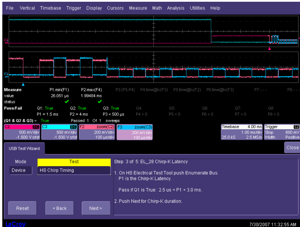
Figure 28. Chirp K Latency
