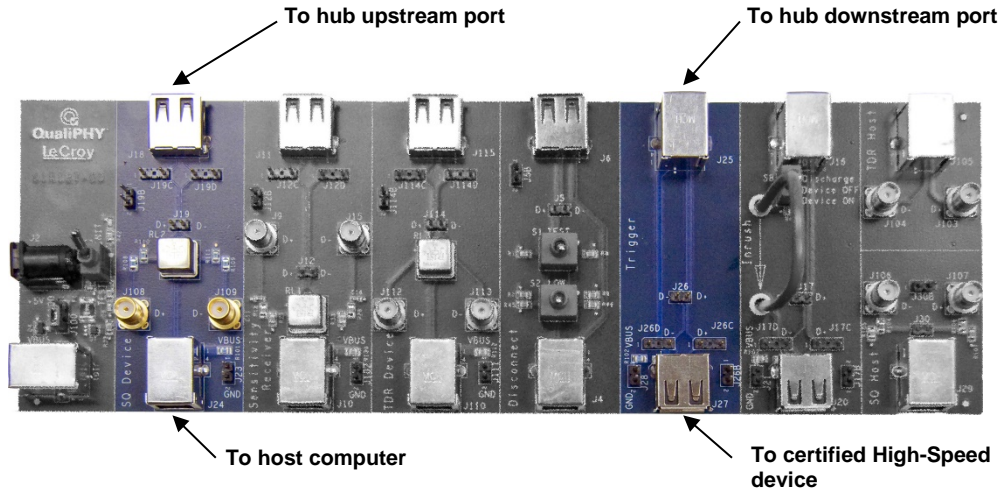
Figure 39. Hub and Device Fixture Connections for Downstream Repeater Test
