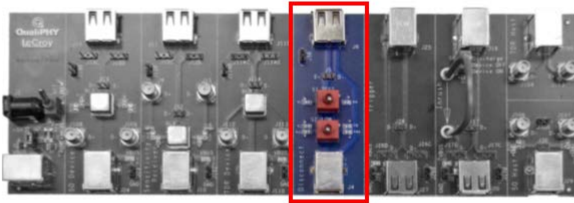
Figure 31. Host Disconnect Section of Test Fixture
