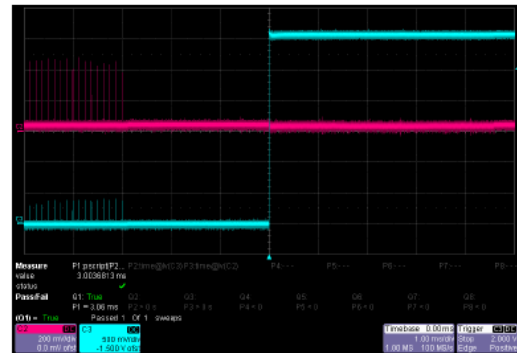
EL_38 HS Suspend Timing Timestamp: 09/25/2007 14:43:42
