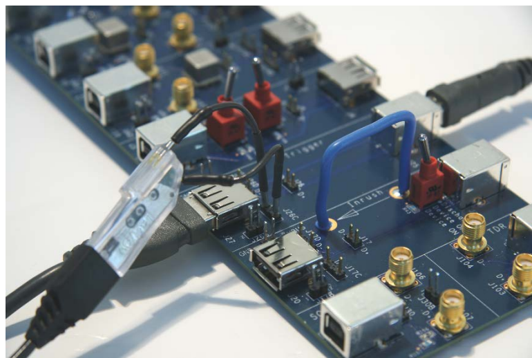
Figure 18. Single-ended Probe Connection Example
