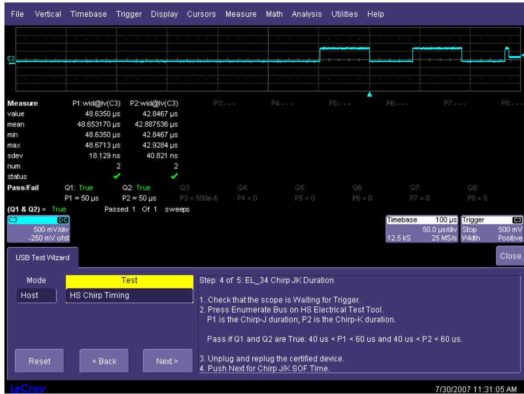
Figure 26. Chirp J and Chirp K Duration
