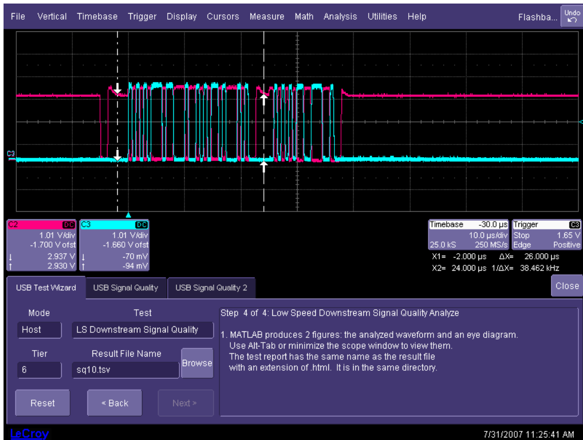
Figure 54. Cursor Positioning for Host Low-Speed Signal Quality Test
