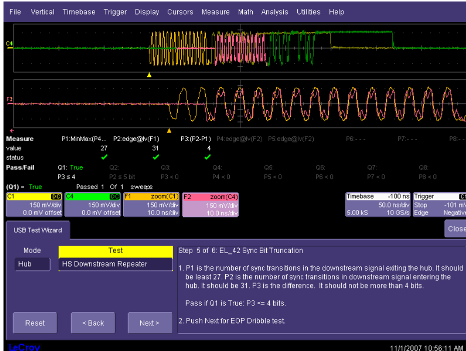
Figure 41. Hub downstream repeater sync field truncation and corruption
