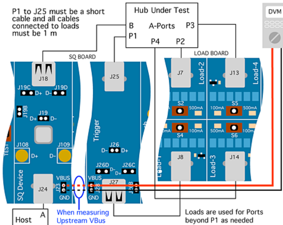
Figure 49. Bus-Powered Hub Drop test equipment setup
