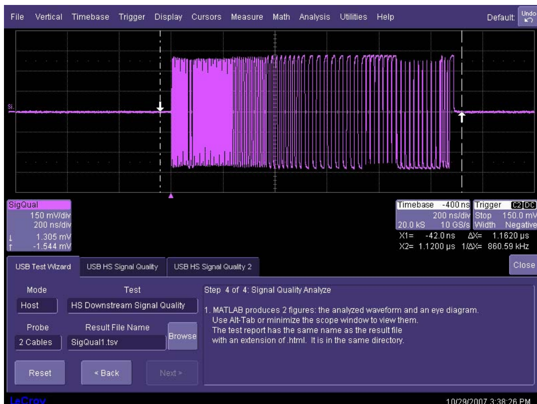
Figure 22. Host High-Speed Downstream Signal Quality Analysis
