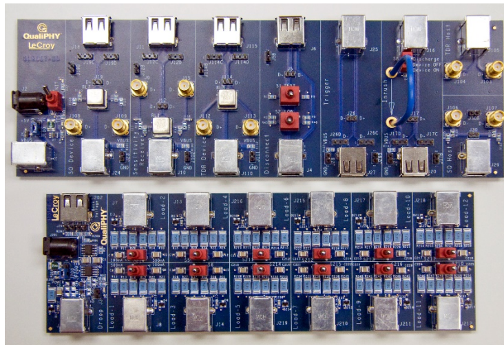
Figure 1. USB 2.0 Test Fixture (Part Number TF-USB-B)
