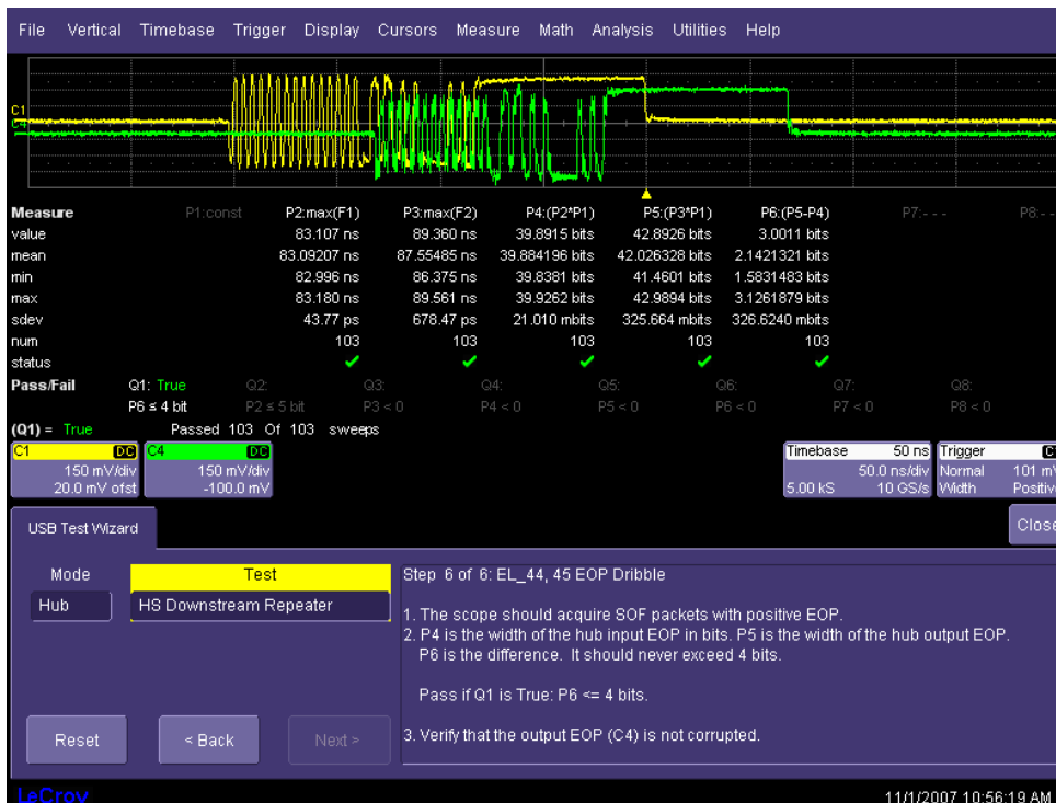
Figure 42. Hub downstream repeater end of packet dribble
