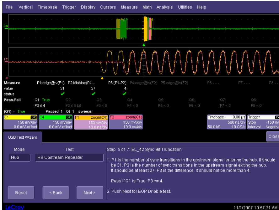
Figure 36. Hub upstream repeater sync field truncation and corruption
