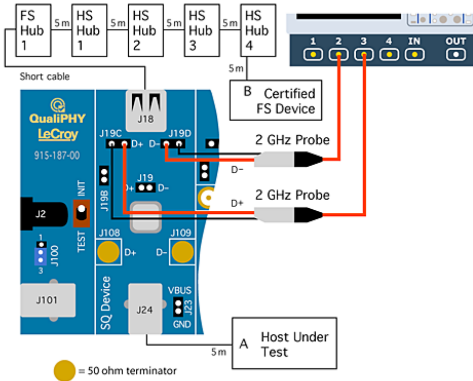
Figure 55. Host Full-Speed Downstream Signal Quality Test Equipment Setup
