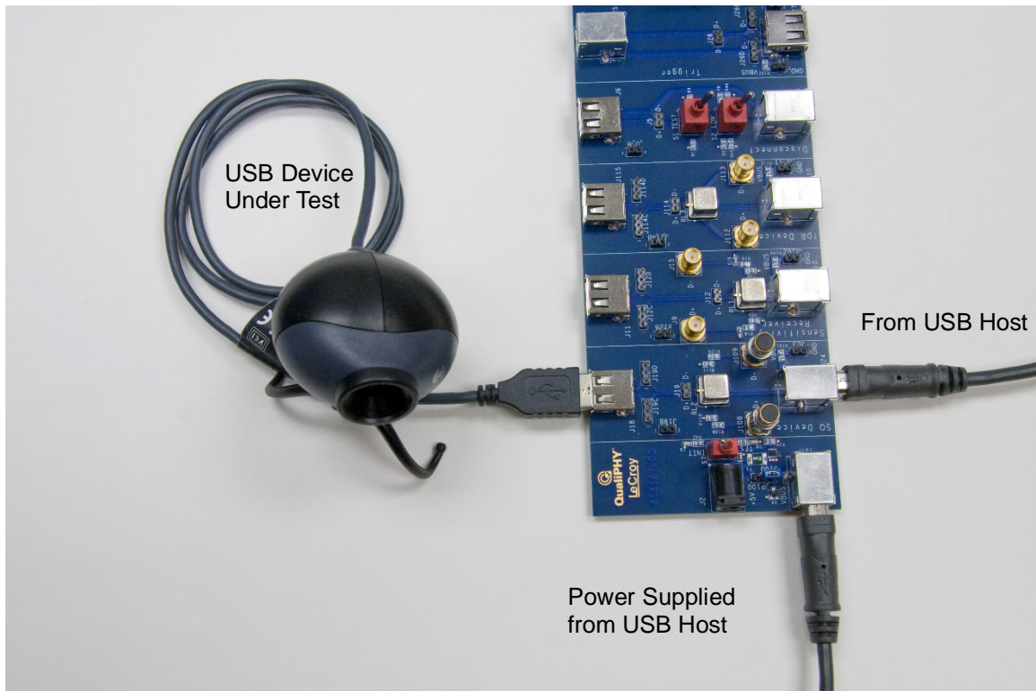
Figure 14. USB camera connected to the Signal Quality section
