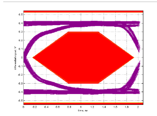
Upstream Eye Diagram, Path on Scope: D:\Applications\USB2 IResults\Qusb8Eye.png Timestamp: 09/25/2007 14:28:46
