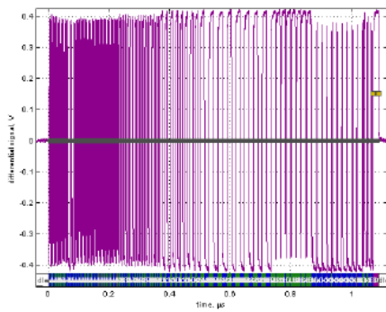
Scope Capture Data Plot, Path on Scope: D:\Applications\USB2 IResults\Qusb8Plot.png Timestamp: 09/25/2007 14:28:47
