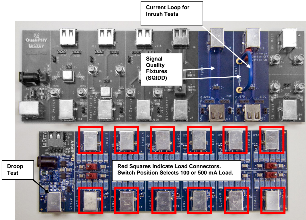
Figure 48. FS/LS Signal Quality Test Fixture Sections
