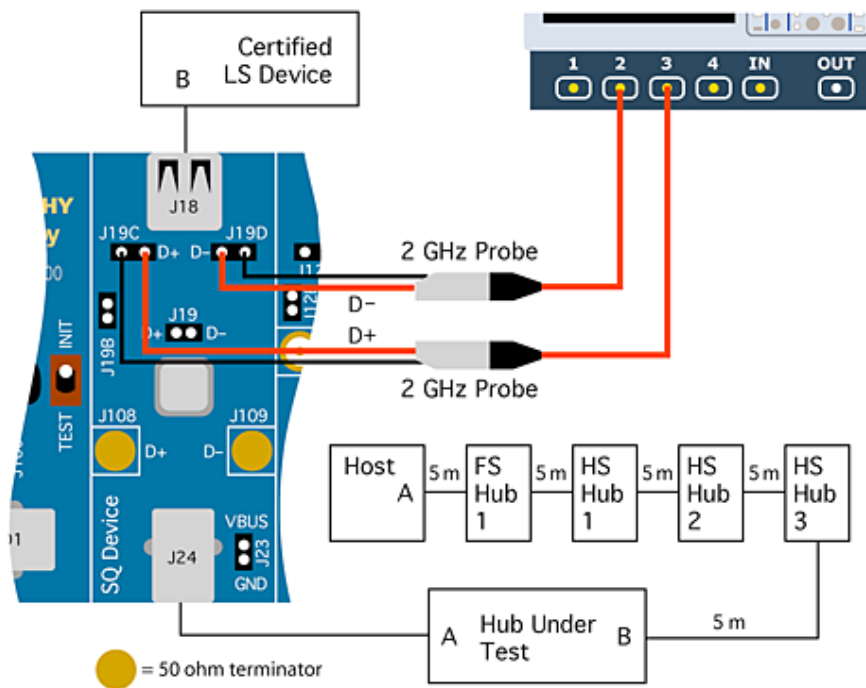
Figure 58. Hub Low-Speed Downstream Signal Quality Setup
