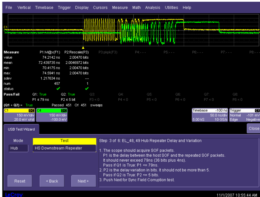
Figure 40. Hub downstream repeater delay
