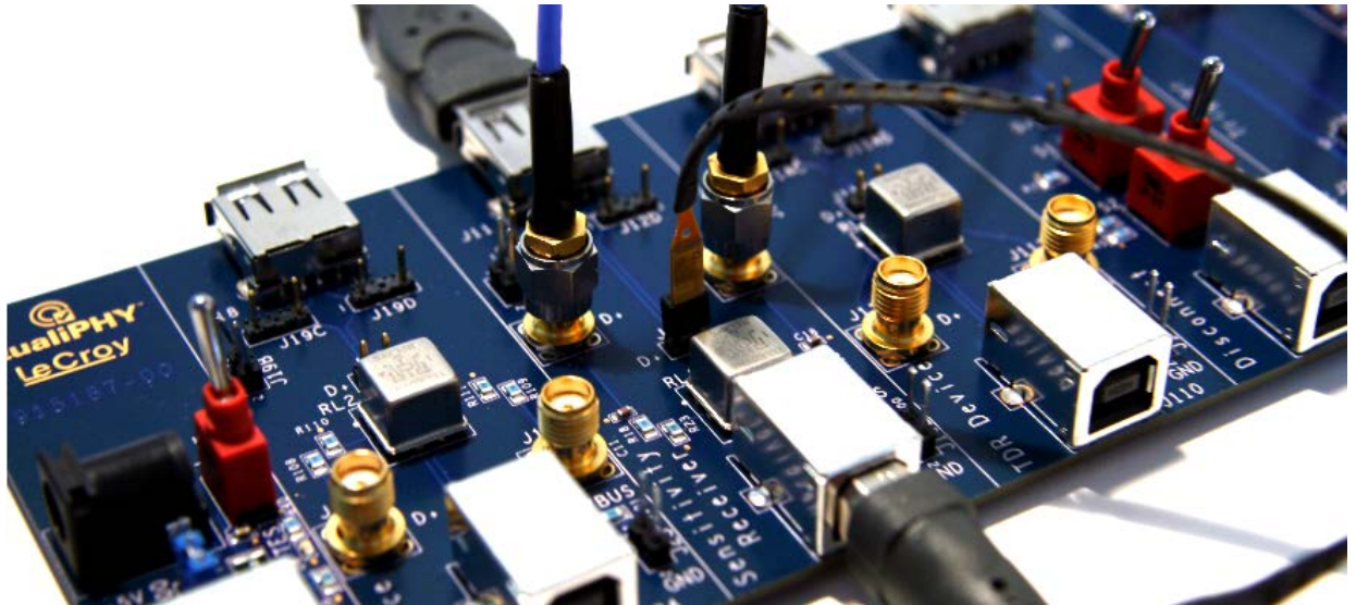
Figure 43. Receiver Sensitivity Test Setup
