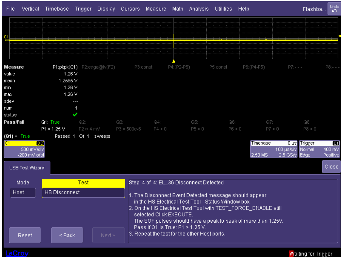
Figure 33. Voltage after disconnect
