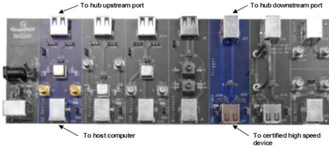
Figure 34. Hub and Device Fixture Connections for Upstream Repeater Test
