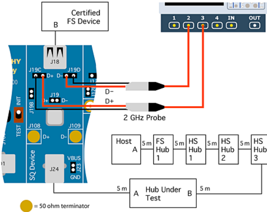
Figure 59. Hub Full-Speed Downstream Signal Quality Setup
