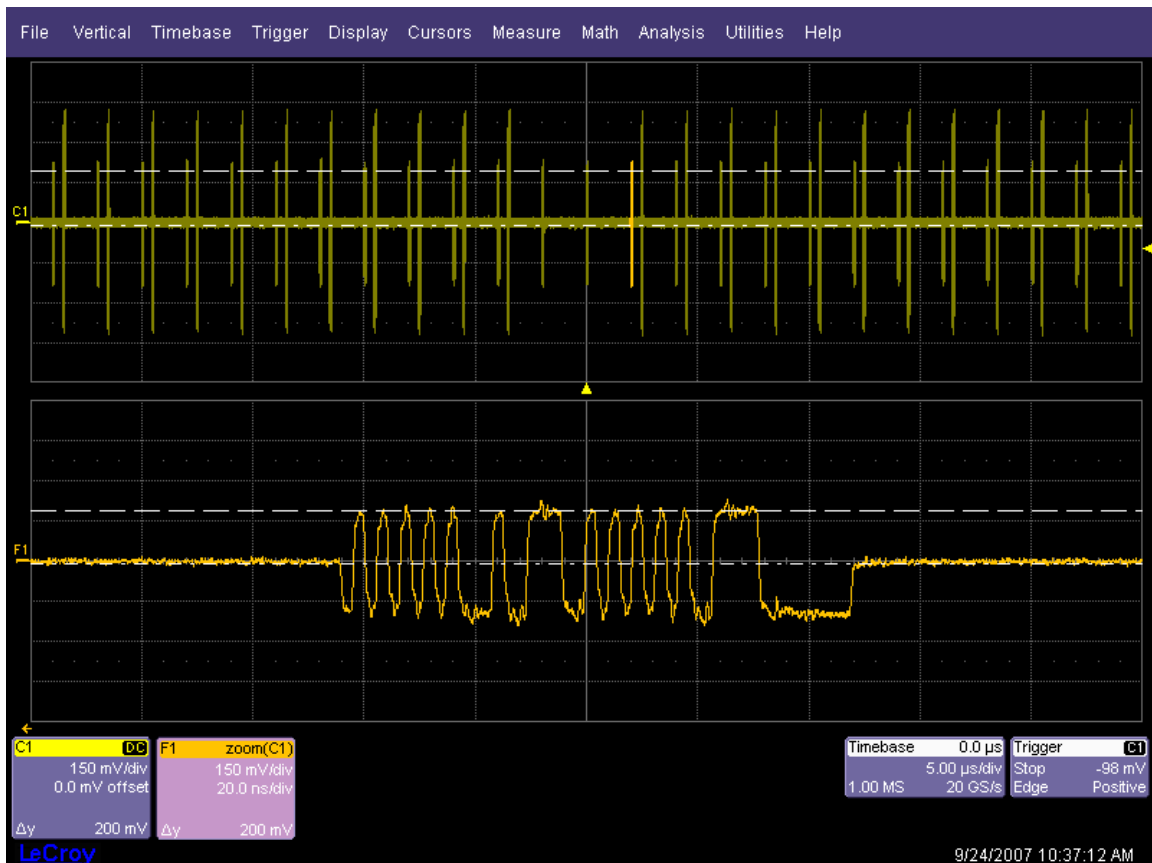
Figure 46. Intermittent Response to IN tokens at low amplitude
