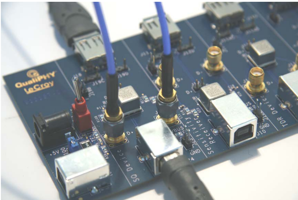
Figure 16. Two SMA Cables Connected to the Test Fixture
