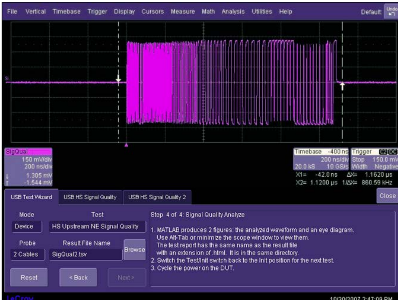
Figure 23. Device High-Speed Upstream Signal Quality
