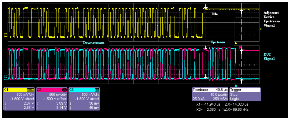
Figure 62. Isolation of Upstream Data Packet
