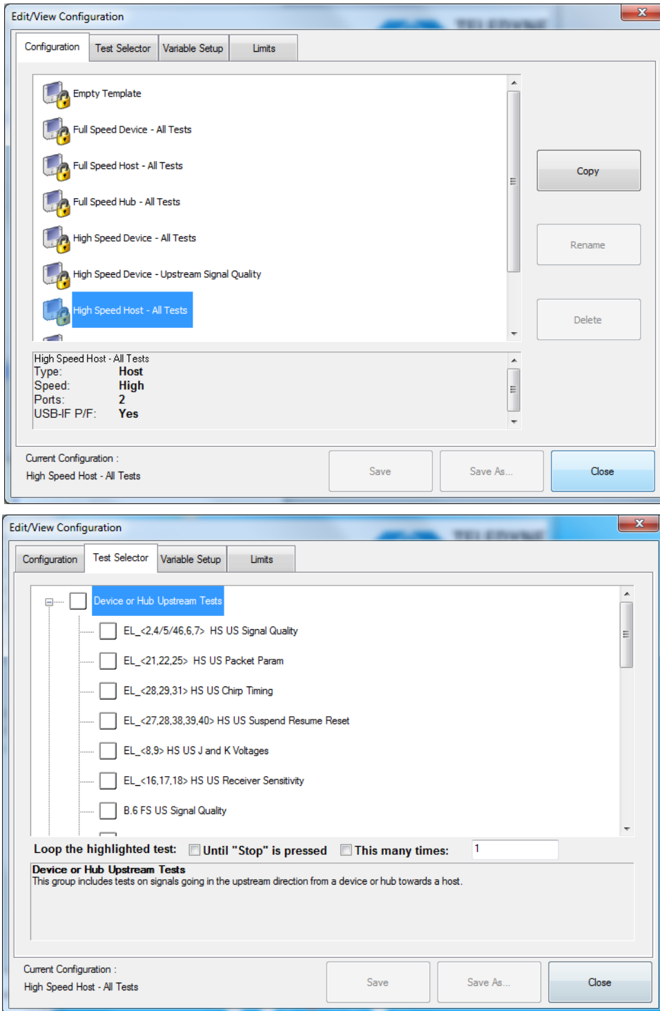
Figure 11. QualiPHY Configuration and Test Selectors
