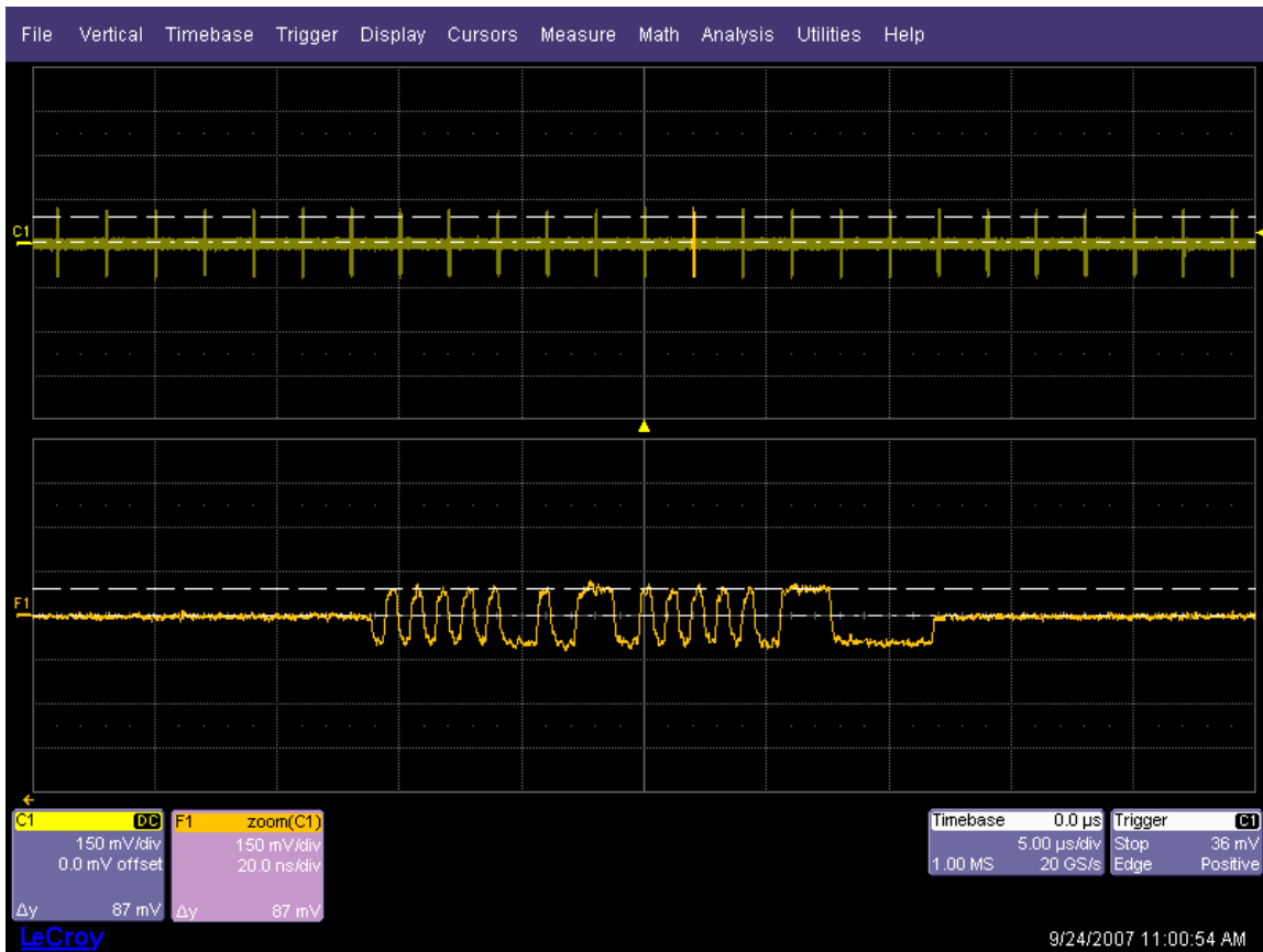
Figure 47. Receiver squelch level – no response to IN tokens
