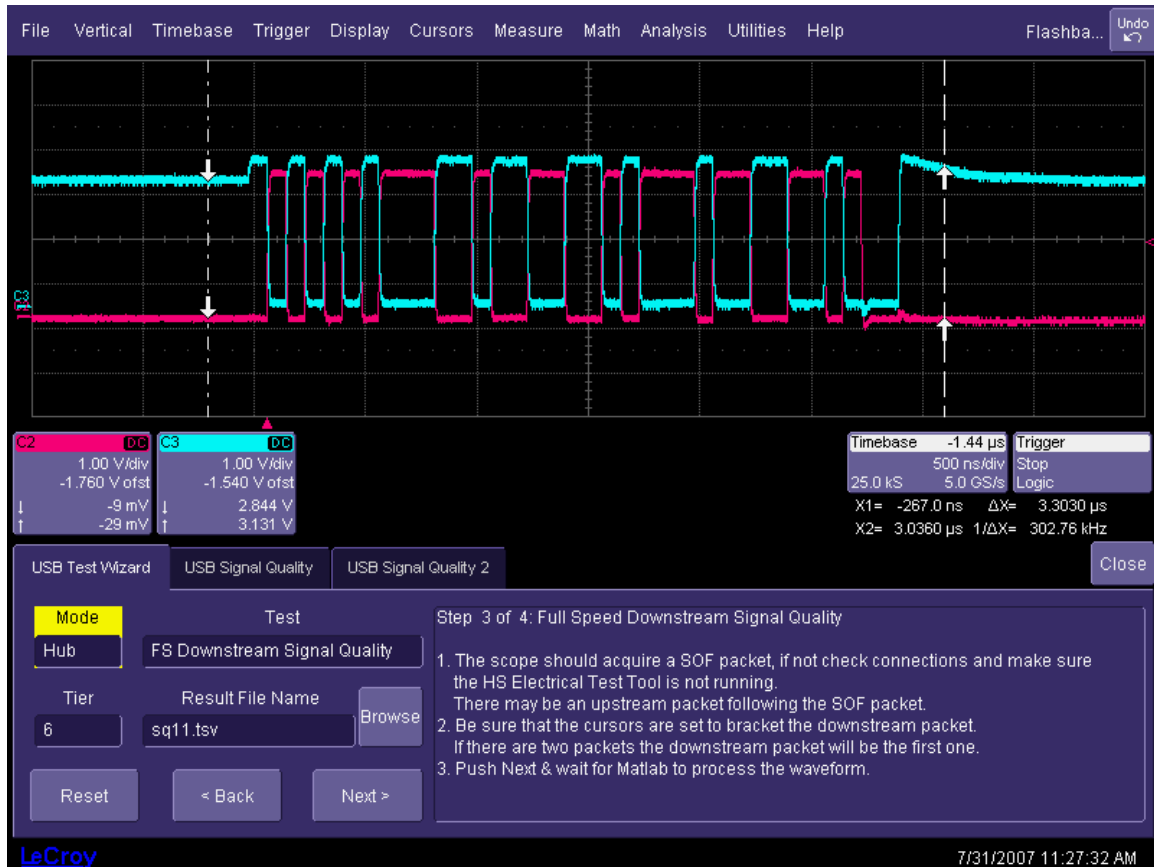
Figure 60. Cursor Placement For Hub FS Downstream Signal Quality Test
