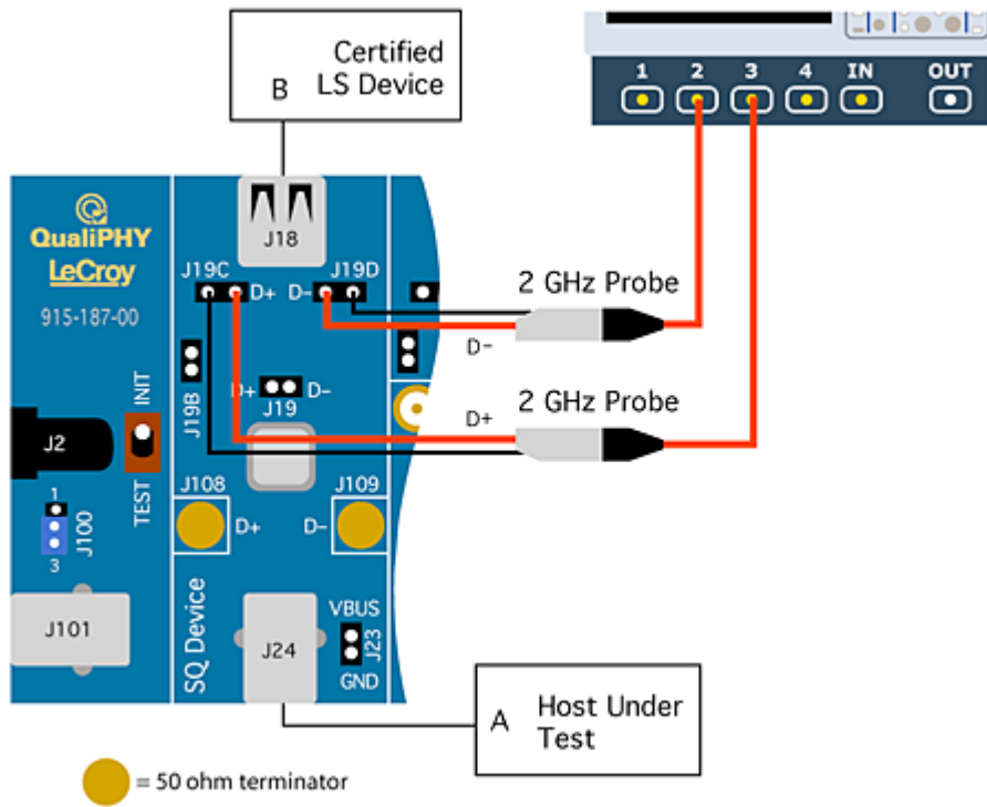
Figure 53. Host Low-Speed Downstream Signal Quality Test Equipment Setup
