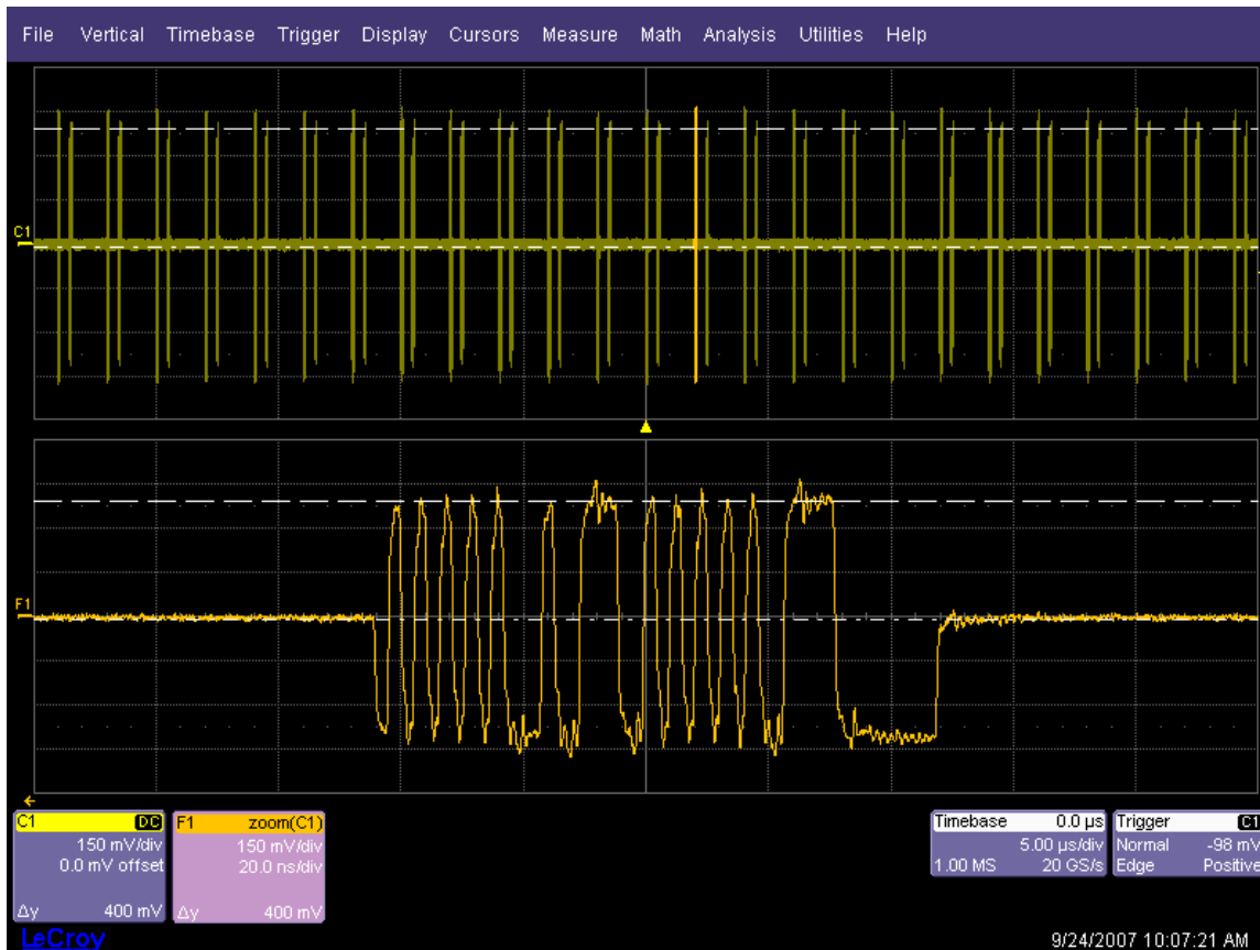
Figure 45. Response to IN tokens with 12-bit sync - all packets NAK'd
