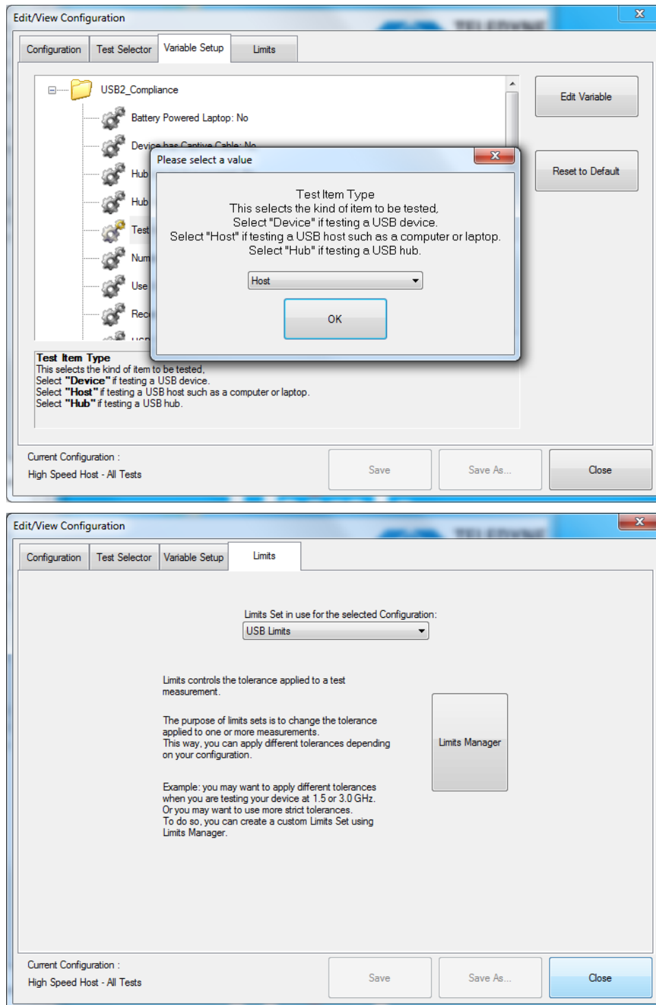
Figure 12. Variable Setup and Limits tabs
