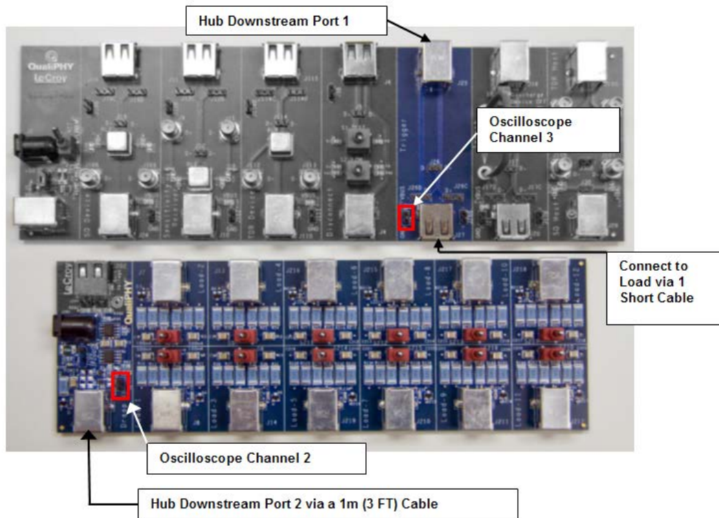
Figure 51. Device and oscilloscope connections for droop test
