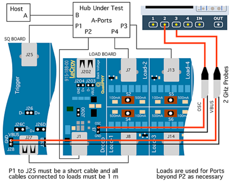
Figure 50. Hub Droop Test Equipment Setup
