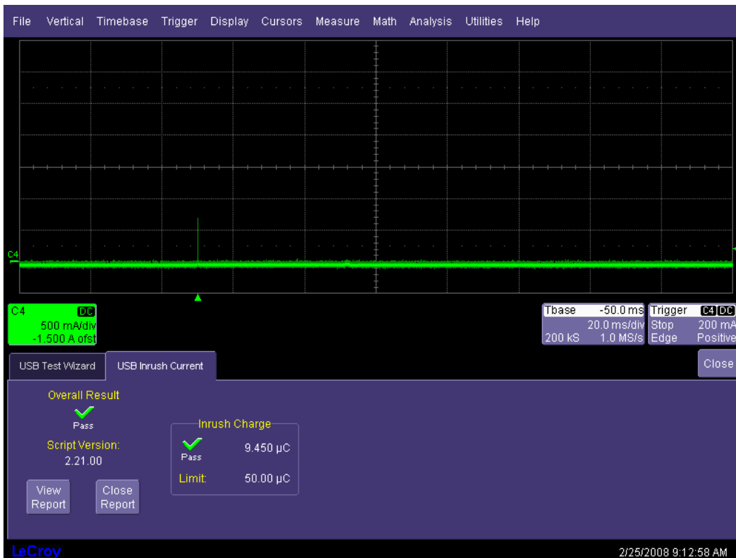
Figure 57. Inrush Current Pulse
