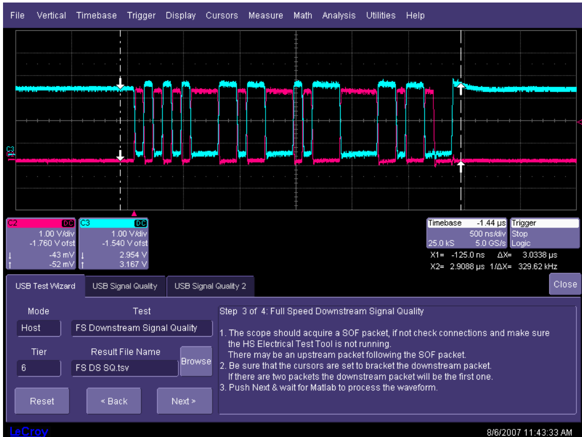
Figure 56. Cursor Positioning for Host Full-Speed Downstream Signal Quality
