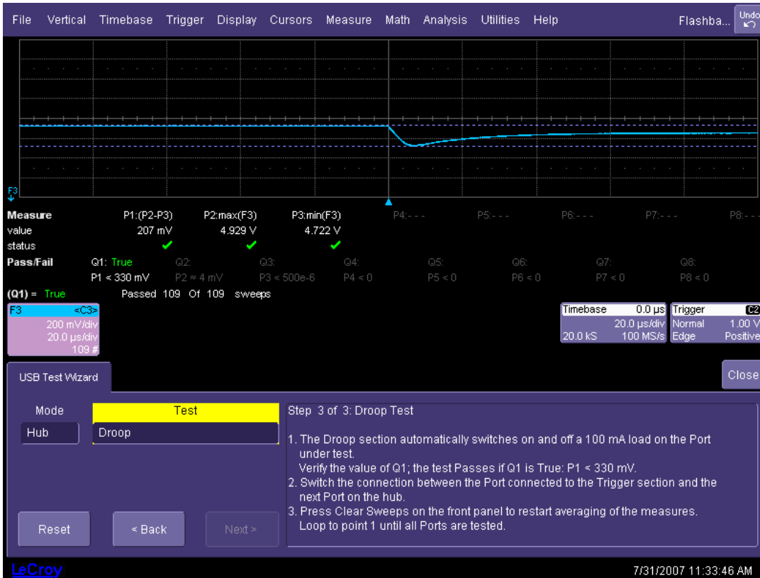
Figure 52. Droop voltage waveform
