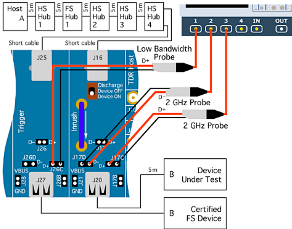
Figure 61. Device Full-Speed Upstream Signal Quality Test Equipment Setup
