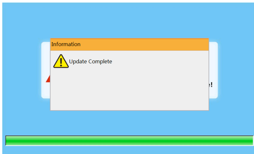
Upgrades interface2
