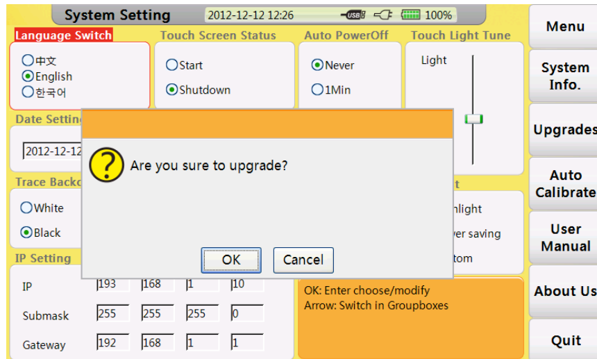
Upgrades interface1
