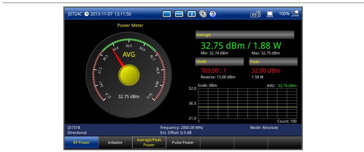
Figure 68 RF power measurement screen
