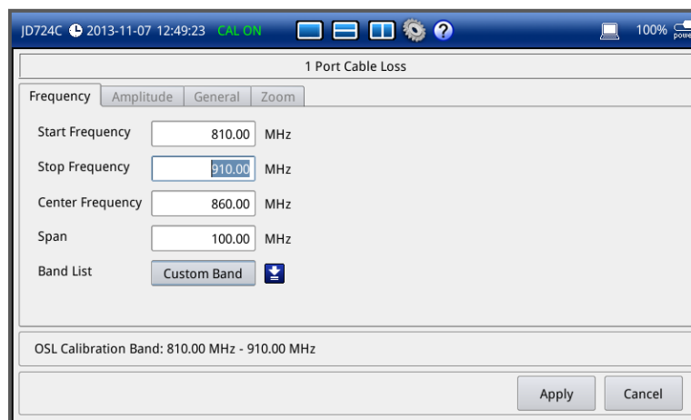
Figure 34 Frequency setup window for cable loss measurements
