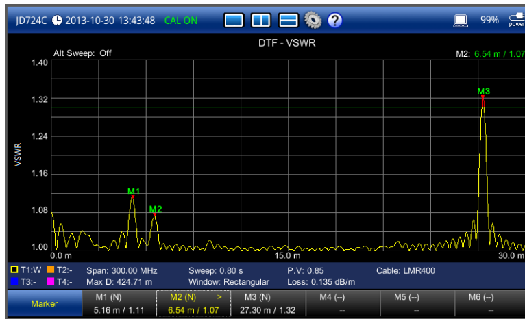
Figure 28 DTF VSWR measurement screen (single layout)
