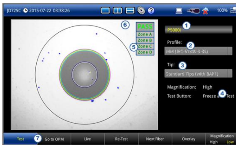
Figure 76 Fiber inspection screen
