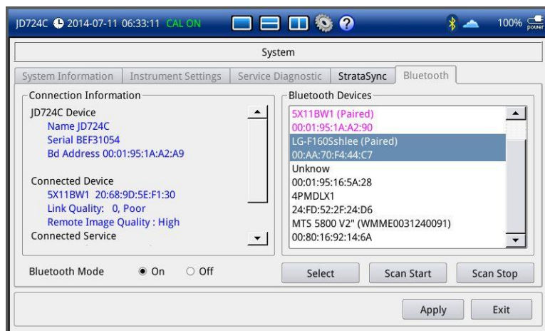
Figure 113 Bluetooth information window
