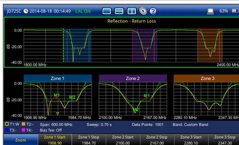
Figure 83 Reflection return loss measurement with zoom zones
