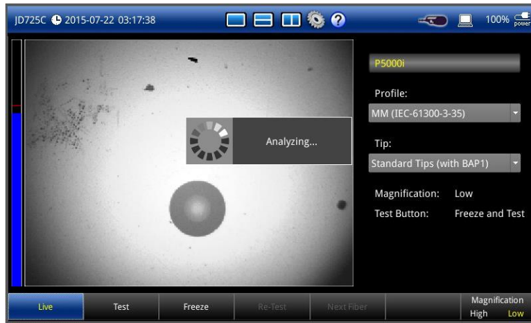
Figure 79 Testing a fiber
