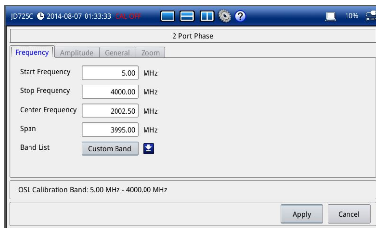
Figure 57 Frequency setup window for 2 port phase measurements
