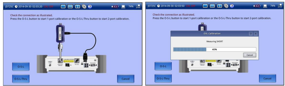
Figure 11 Electronic calibration on JD725C using EZ-Cal kit
