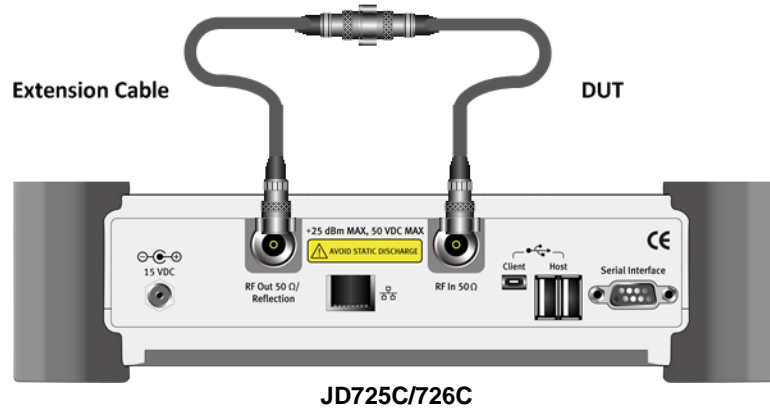
Figure 59 Connection diagram for 2-port phase measurements
