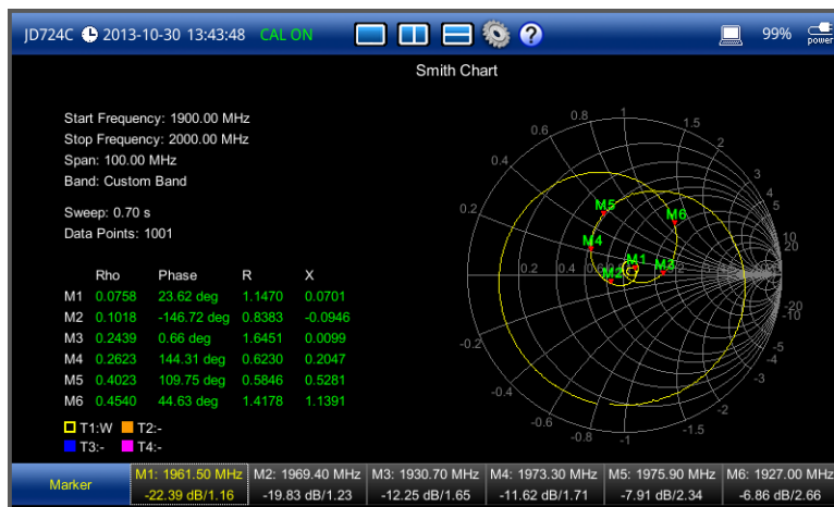
Figure 48 Smith chart measurement screen (single layout)
