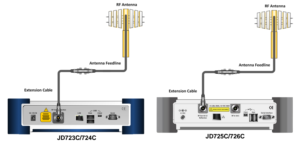
Figure 42 Cable connection diagram for 1 port phase measurements
