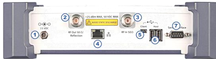
Figure 3 JD725C Top panel view
