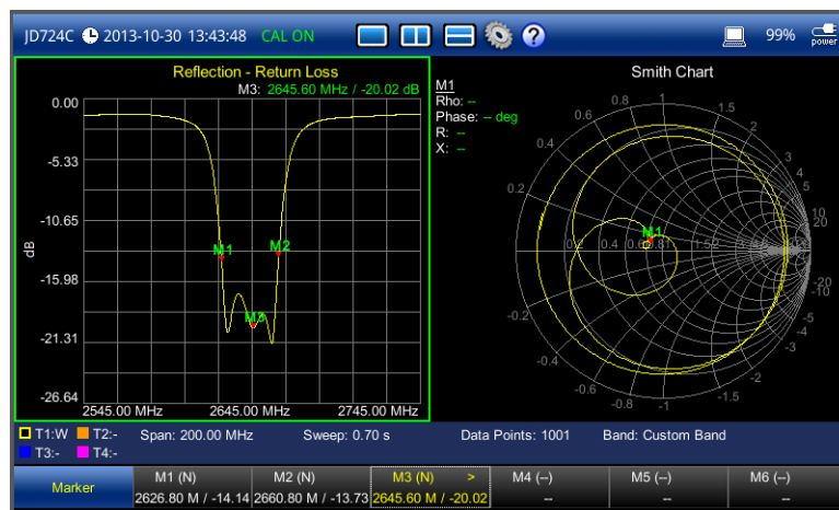
Figure 23 Reflection return loss & smith chart measurement screen (vertical layout)
