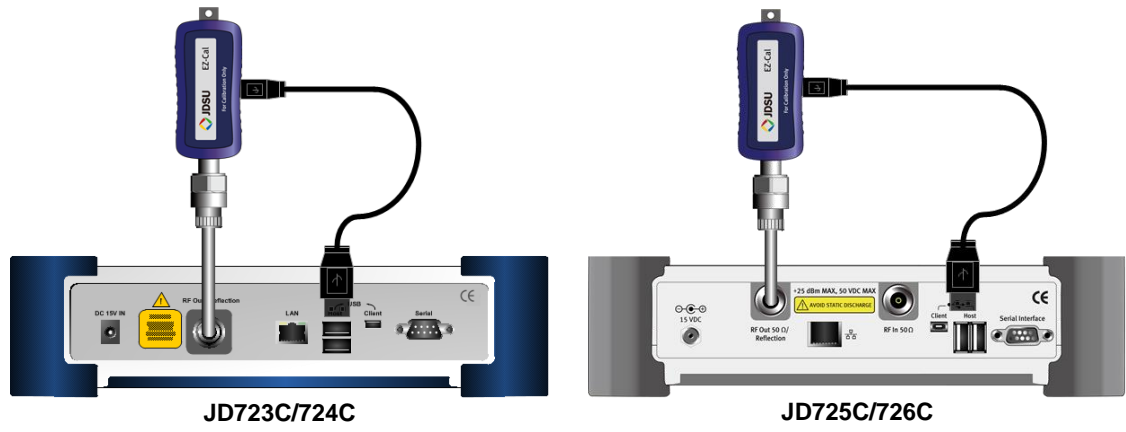
Figure 9 e-Calibration connection diagram with an extension cable
