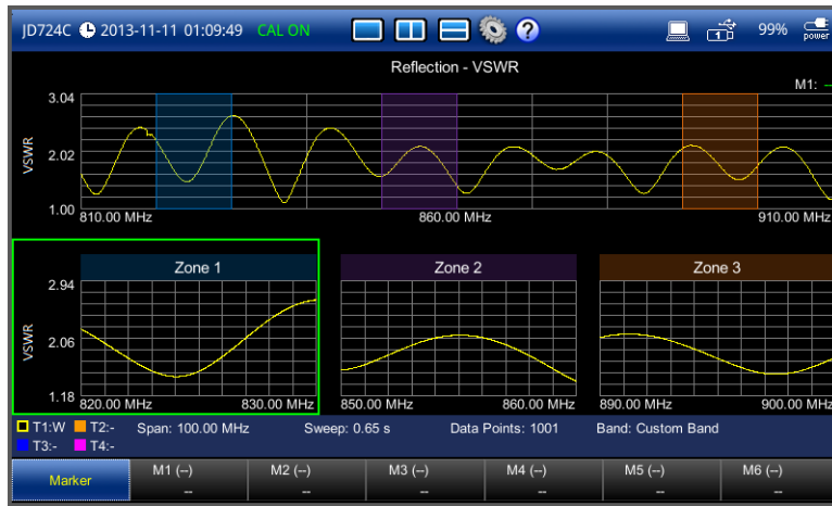
Figure 19 Reflection VSWR measurement screen (zoom zones)
