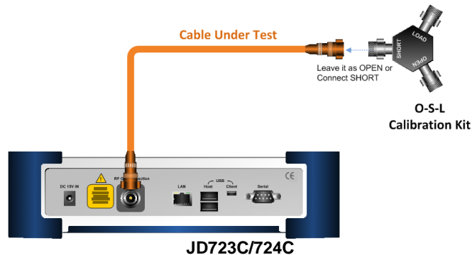
Figure 36 Cable connection diagram for cable loss measurements
