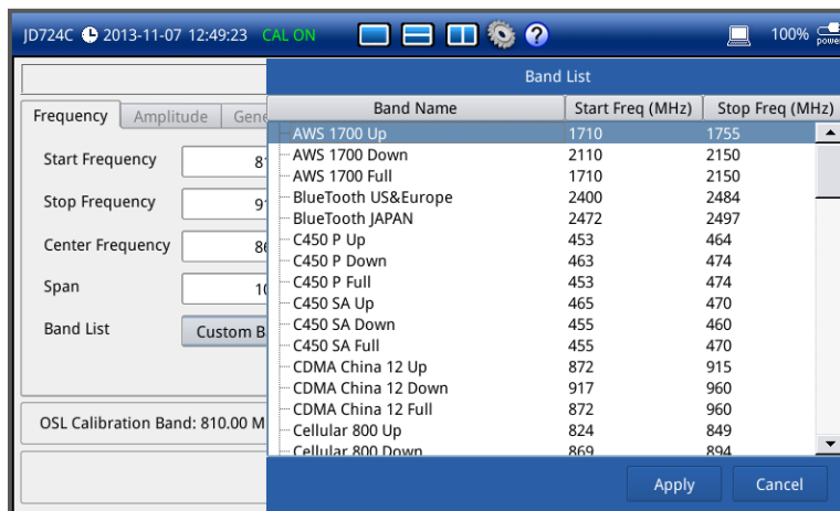
Figure 58 Band list window
