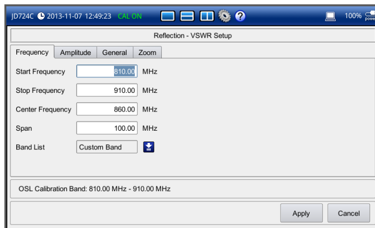
Figure 15 Frequency setup window for reflection measurements
