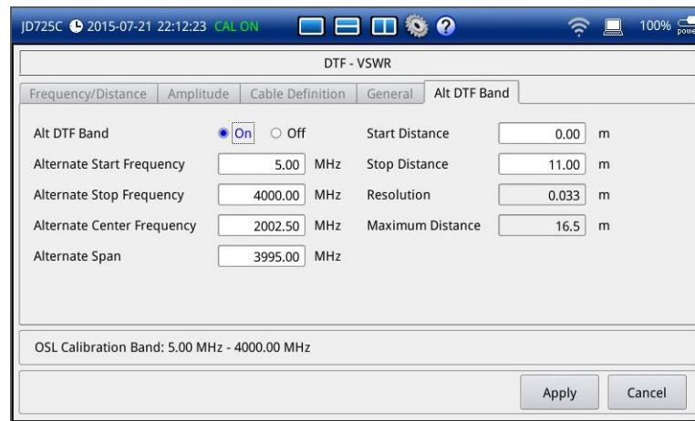
Figure 84 Alternate DTF band setting window
