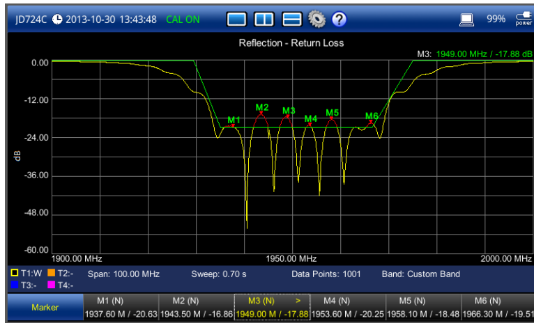
Figure 20 Reflection return loss measurement screen (single layout)
