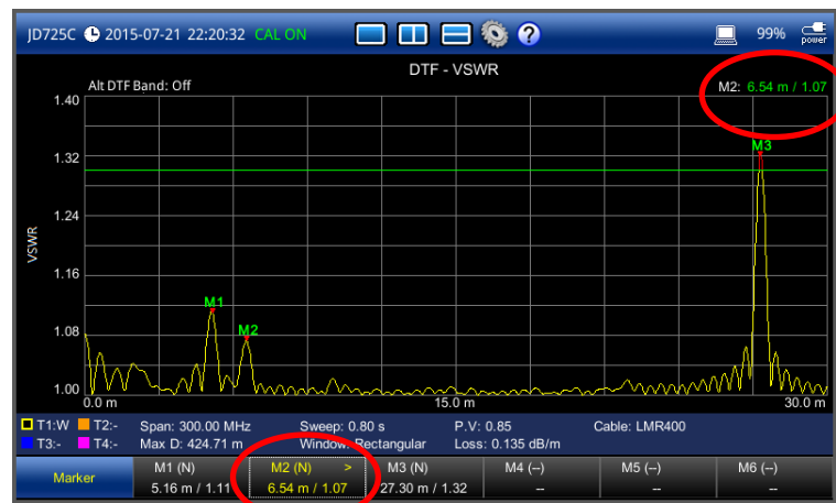
Figure 86 Active marker and its readout
