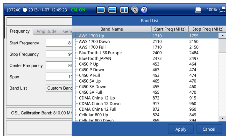
Figure 16 Band list window
