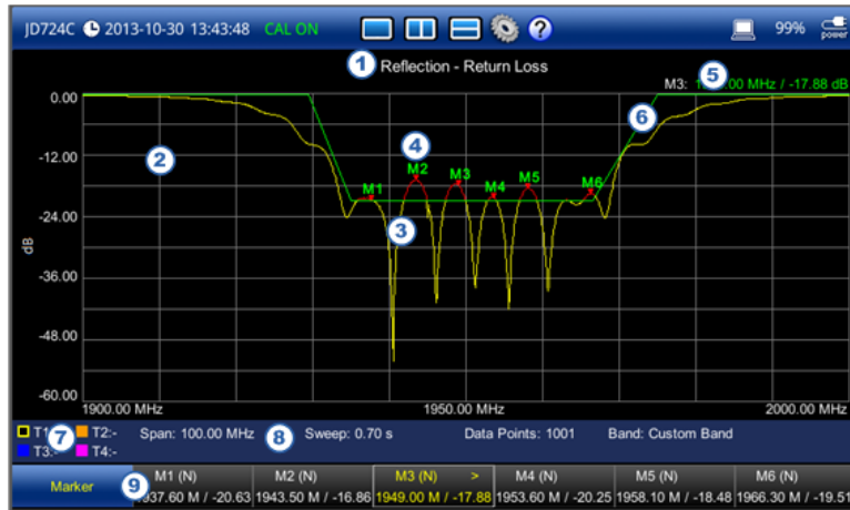
Figure 14 Reflection measurement screen
