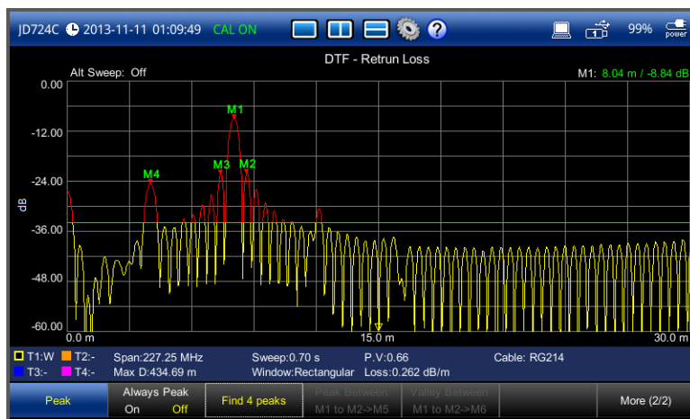
Figure 29 DTF return loss measurement screen (single layout)
