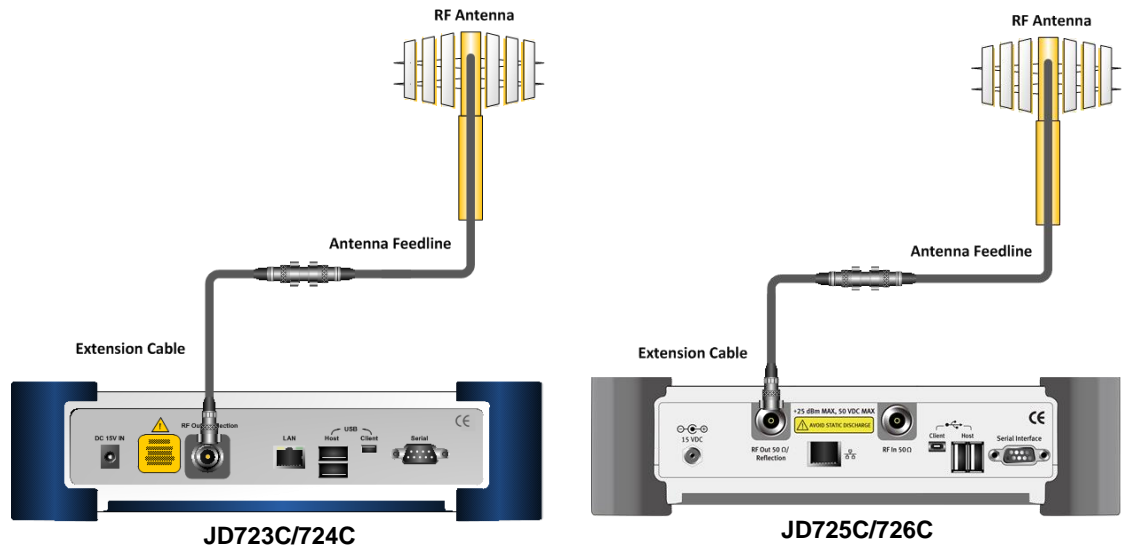
Figure 47 Cable connection diagram for Smith chart measurements
