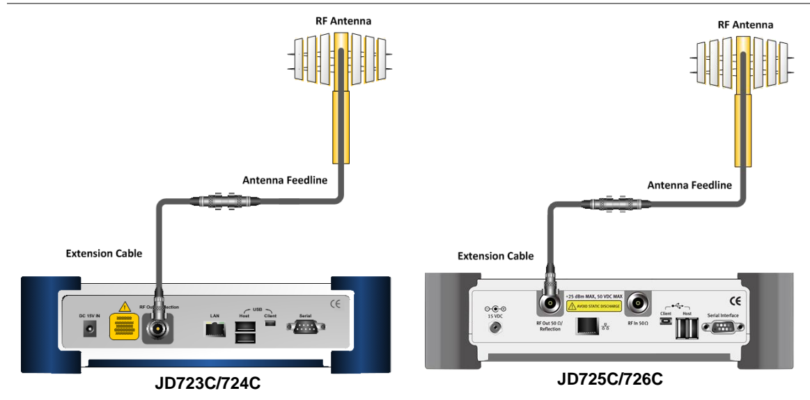
Figure 17 Cable connection diagram for reflection measurements
