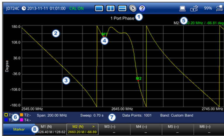
Figure 39 1 port phase measurement screen
