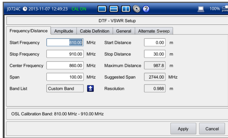
Figure 25 Frequency/distance setup window for DTF measurements
