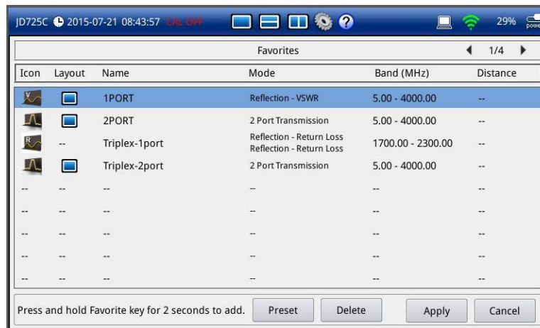
Figure 95 Favorites window
