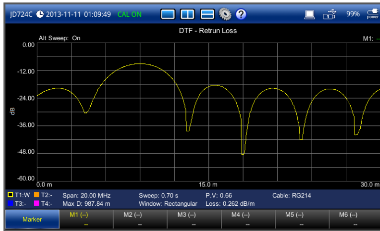
Figure 30 DTF return loss measurement screen (alternate sweep on)
