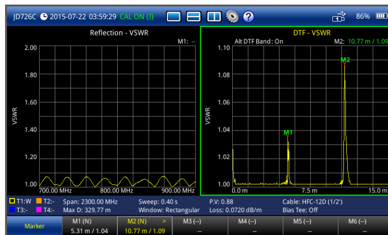
Figure 85 DTF VSWR measurement with alternate DTF band on
