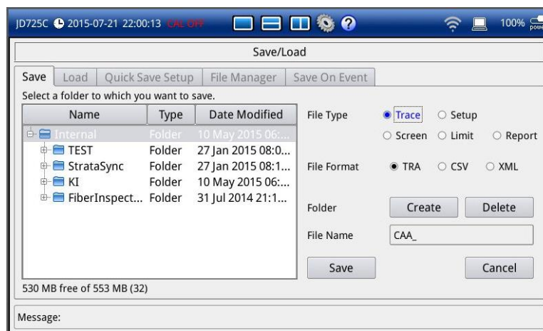
Figure 91 Save window
