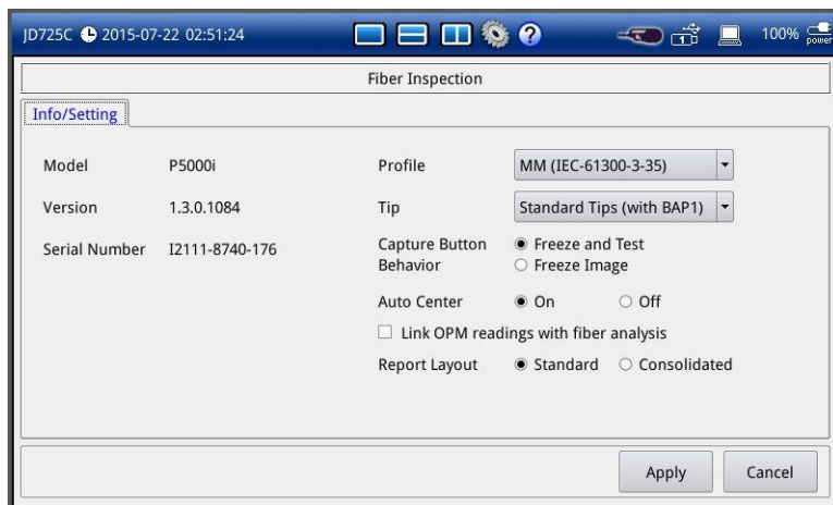
Figure 77 Info/Setting window
