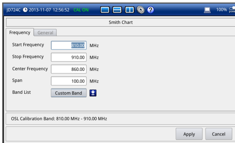
Figure 45 Frequency setup window for Smith chart measurements
