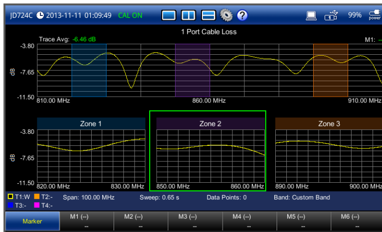
Figure 38 1 port cable loss measurement screen (zoom zones)
