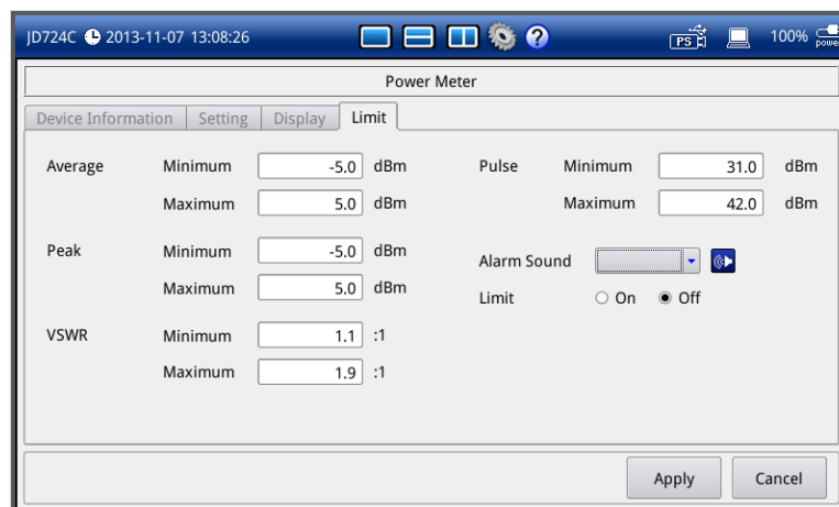
Figure 69 Limit setup window for RF power measurements
