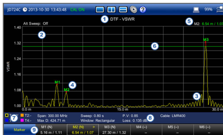
Figure 24 DTF measurement screen
