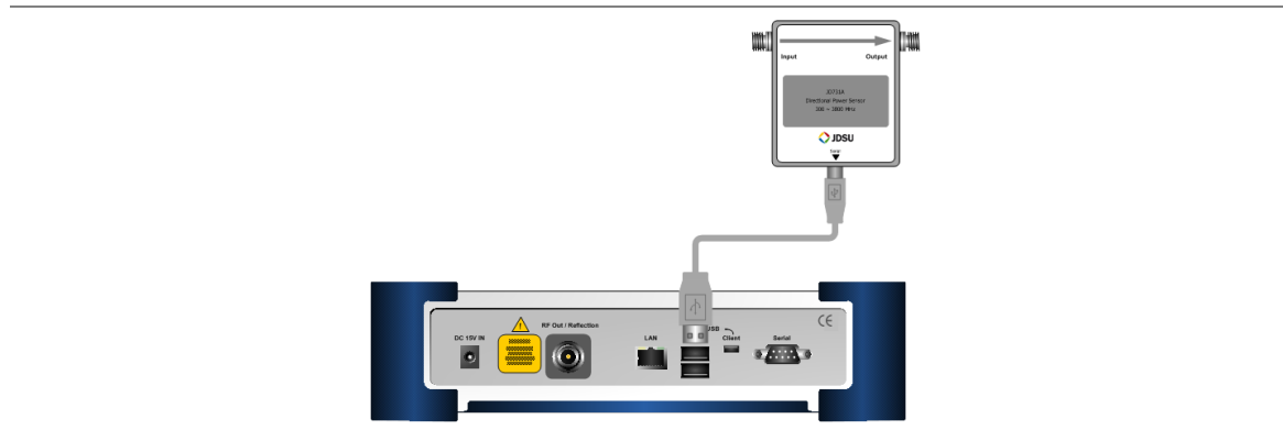
Figure 67 Cable connection diagram for directional power sensor
