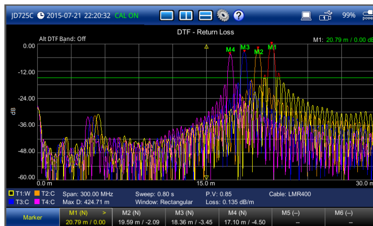
Figure 87 Trace overlay example
