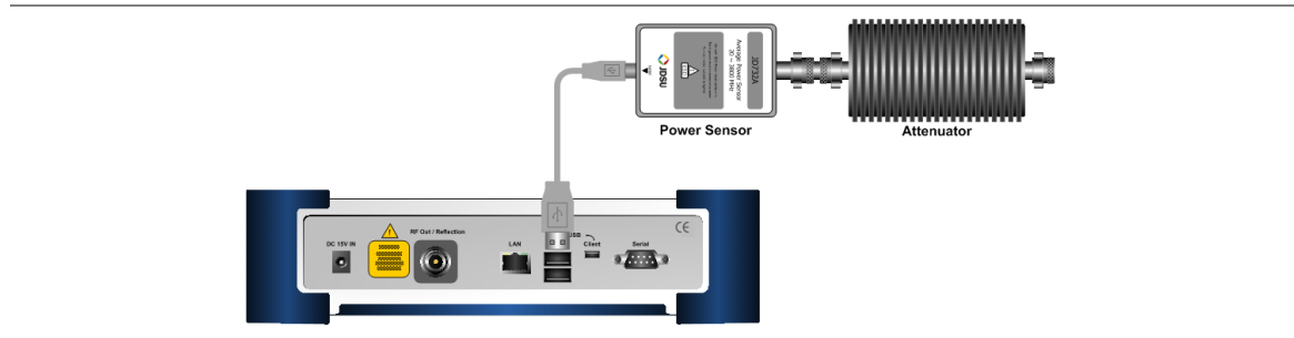
Figure 66 Cable connection diagram for terminating power sensor
