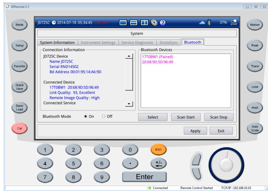
Figure 112 JDRemote screen
