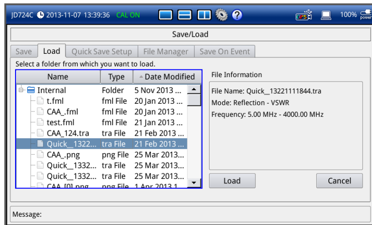
Figure 94 Load window
