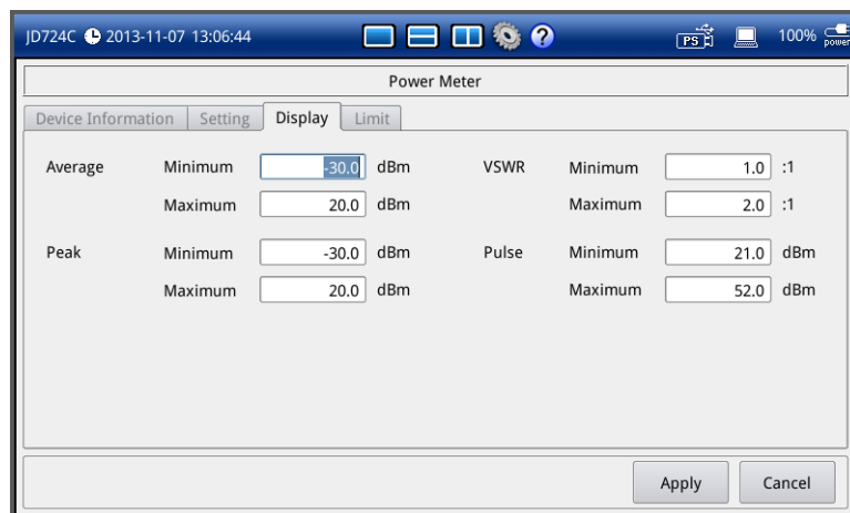
Figure 65 Display setup window for RF power measurements
