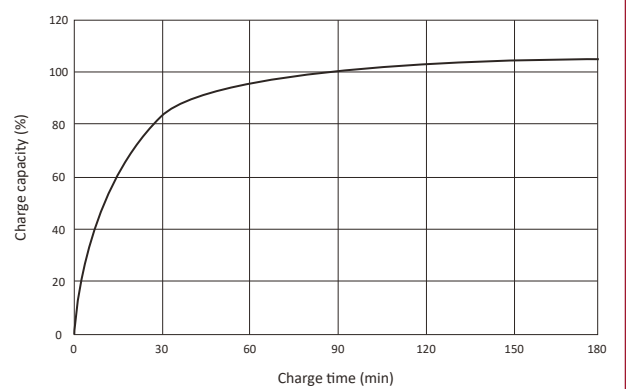
Quick Charge Performance Curve
