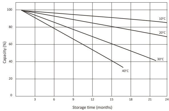
Curve of Self-discharge at Different Temperature
