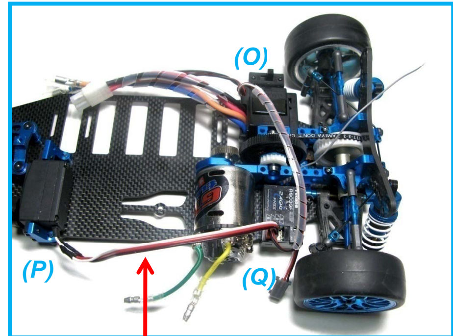
Place black plug from servo motor (P) into socket “1” of receiver (Q)
